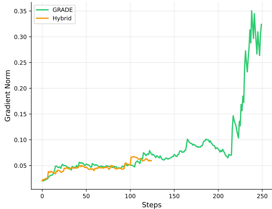
(a) Gradient Norm Over Training
